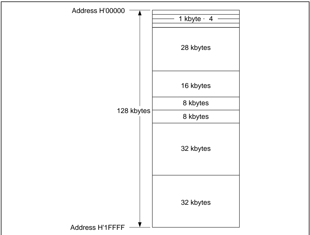
Figure 20.5 Block Configuration
