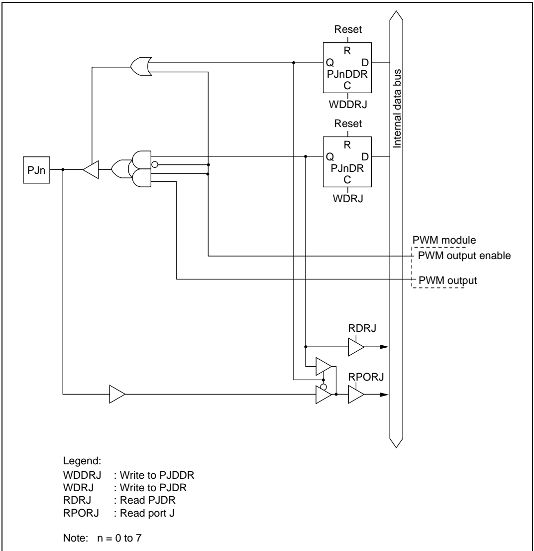
Figure C.14 Port J Block Diagram (Pins PJ0 to PJ7)
