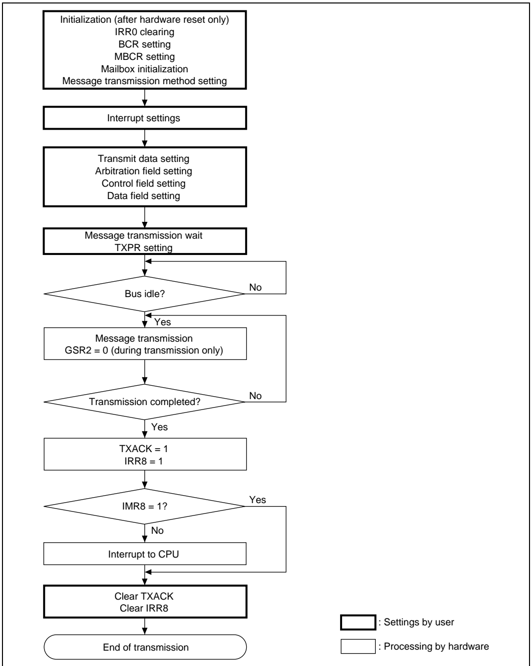
Figure 15.7 Transmission Flowchart
