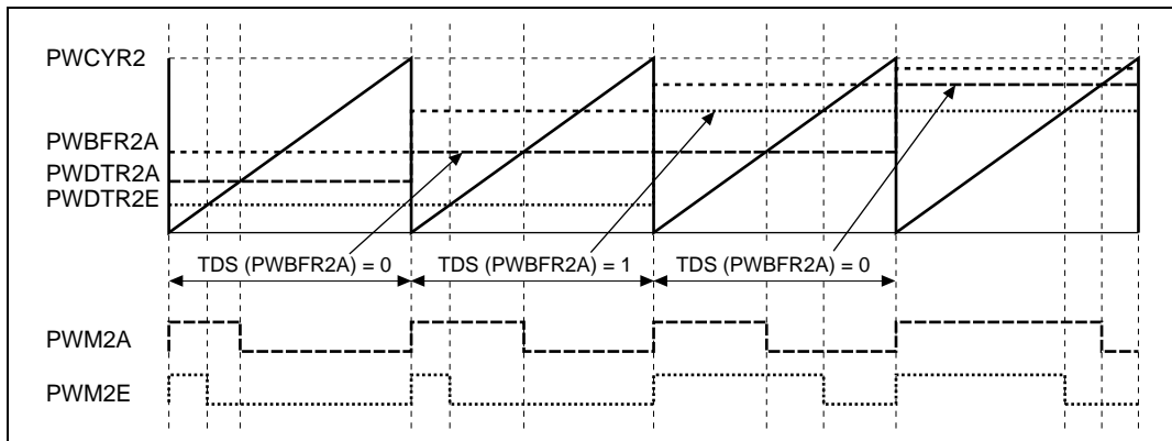
Figure 17.11 PWM Channel 2 Operation
