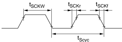
Figure 23.17 SCK Clock Input Timing
