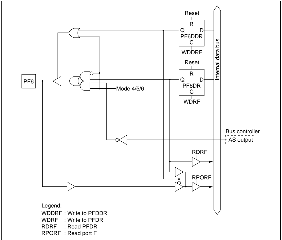
Figure C.12 (f) Port F Block Diagram (Pin PF6)
