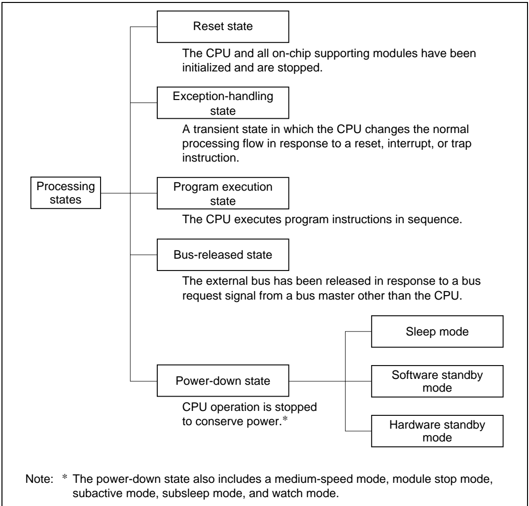
Figure 2.14 Processing States
