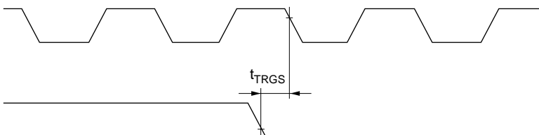
Figure 23.19 A/D Converter External Trigger Input Timing
