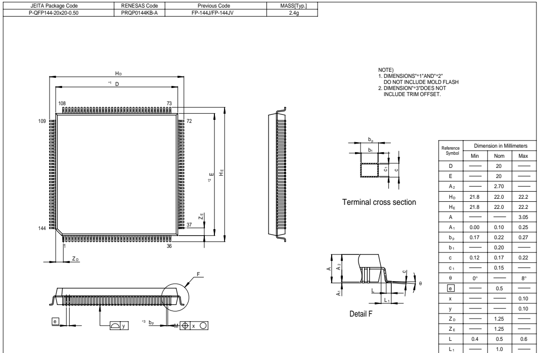
Figure F.1 FP-144J Package Dimension (H8S/2646R, H8S/2648R)
